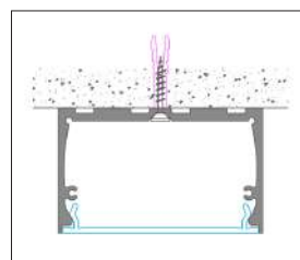
MONTAGGIO A PARETE WALL-MOUNTED
